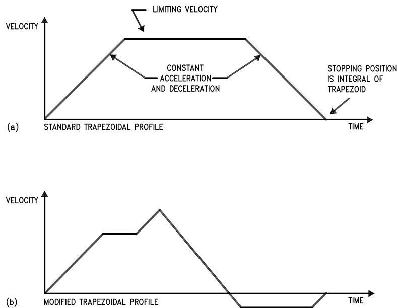
FIGURE 10. Typical Velocity Profiles
